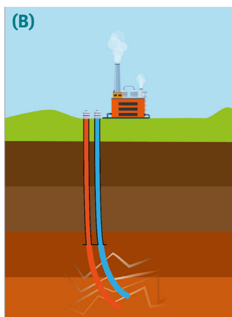
Research fields in geothermal scientific drilling (A) Supercritical and Ultra High Temperature Systems, (B) Enhanced Geothermal Systems, (C) Low to Mid Enthalpy Systems
