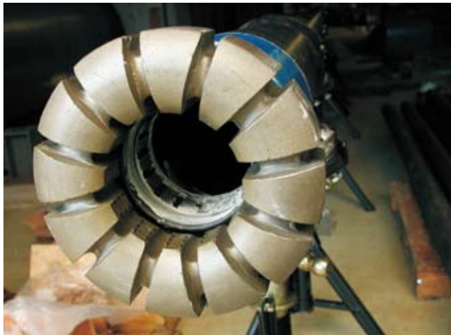
Figure 2. The core bit and core catcher assembly.
