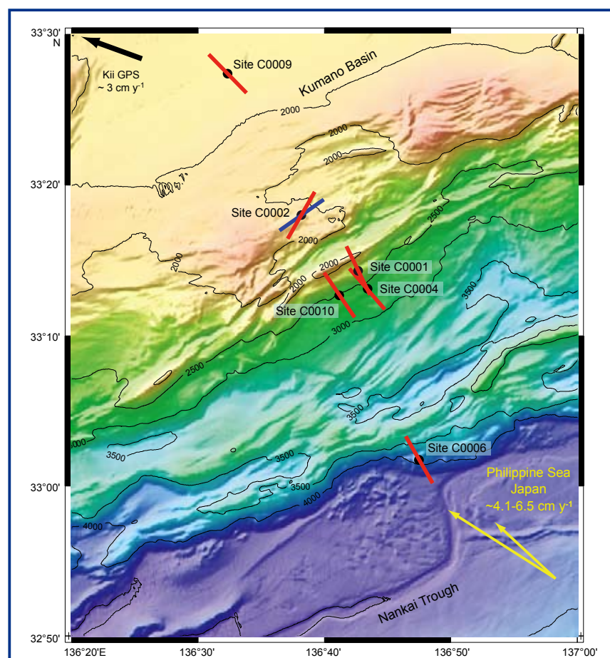
Figure 6. Map showing orientations of maximum horizontal stress inferred from borehole breakouts (see also Kinoshita et al., 2009a). At Site C0002, red line = orientation in forearc basin sediments, blue line = orientation in underlying accretionary prism. Yellow arrows indicate range of suggested convergence rates between the two plates and black arrow indicates GPS-constrained displacement on the Kii peninsula (Seno et al., 1993; Miyazaki and Heki, 2001; Heki, 2007).
