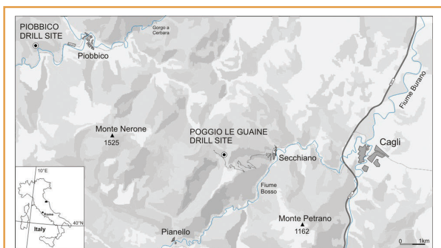
Figure 1. Location of the Poggio le Guaine drill site in the Umbria-Marche Basin (northern Apennines, central Italy). The location of the Piobbico drill site—where an 84-m-thick core extending from the upper Albian down to the uppermost Barremian was drilled in 1982—is also shown.
